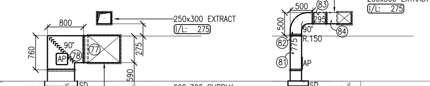
DETAIL G
