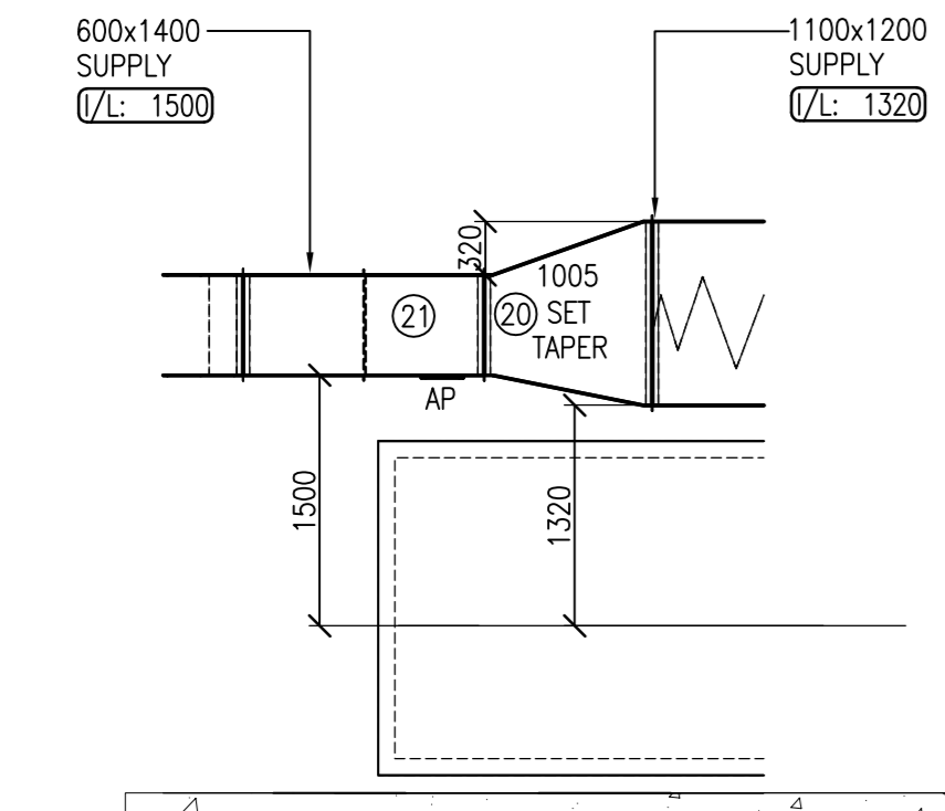
DETAIL F
