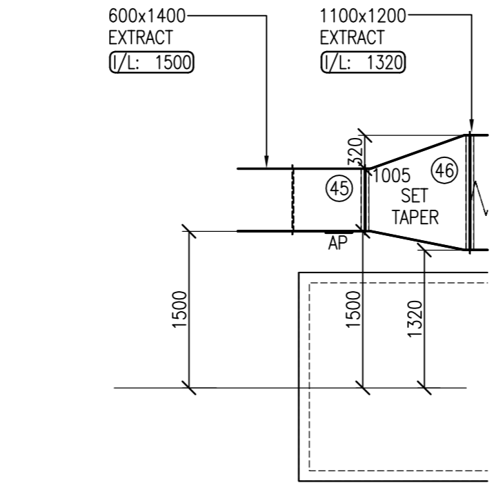
DETAIL E
