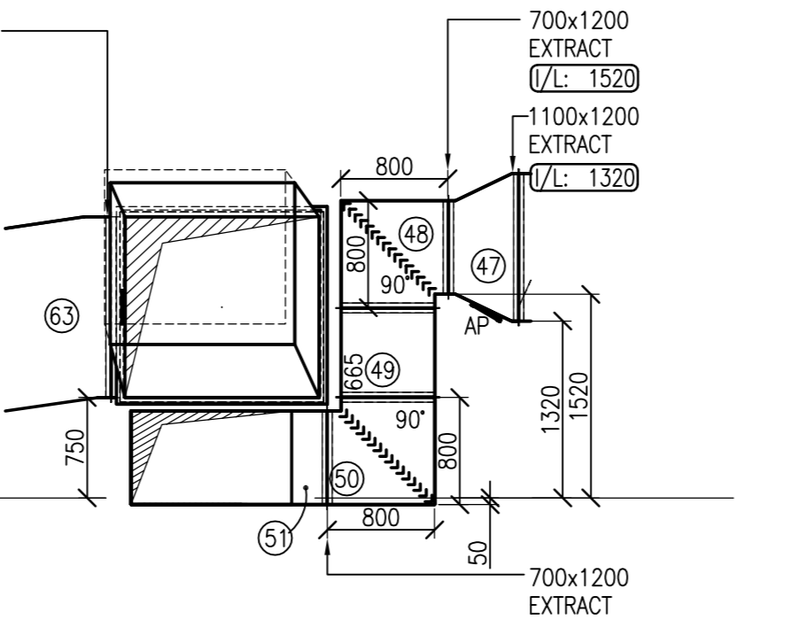
DETAIL D
